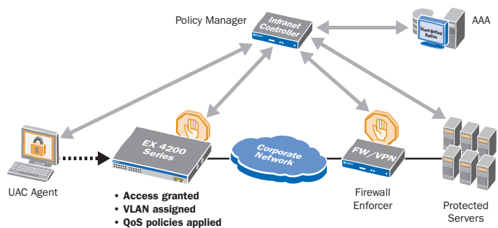
Figure 4: The EX 4200 series switches work with the Juniper UAC solution to enforce access control down to the individual port level.
